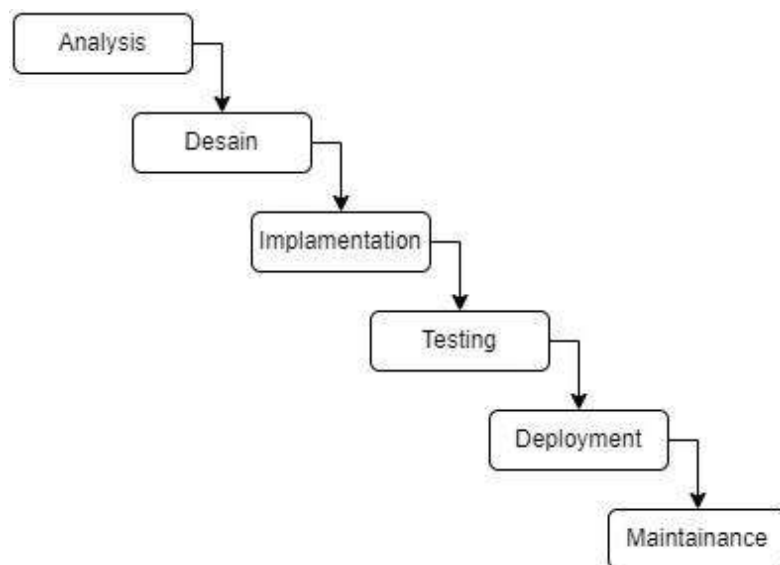
Gambar 3.1 Model Waterfall
