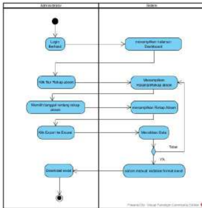
Gambar 5.19 Activity Diagram Rekapitulasi Data Kehadiran
