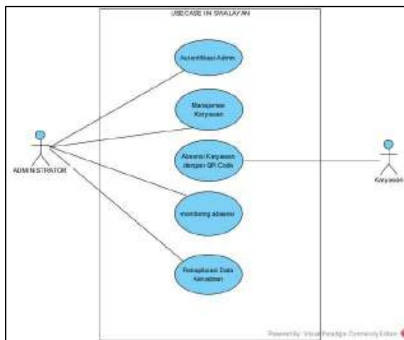
Gambar 5.2 Use Case Diagram
