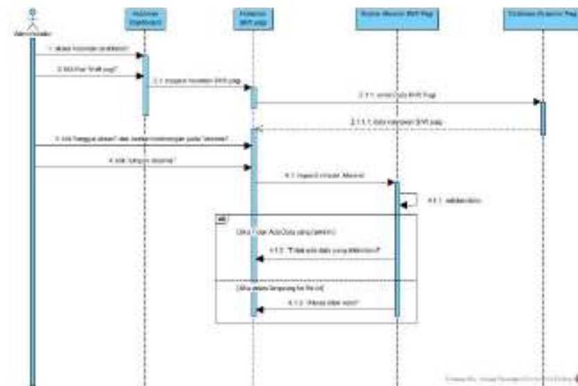
Gambar 5.9 Sequence Diagram Pencatatan Absensi Karyawan E-1
